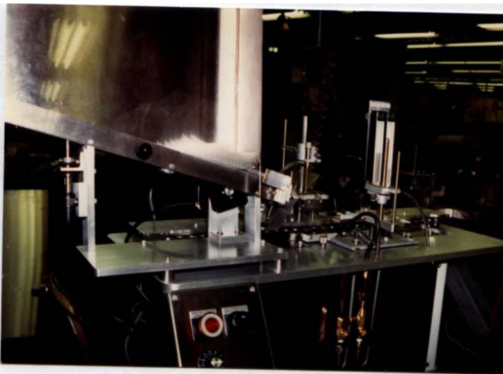
FPS 10S with auto tube feeder
